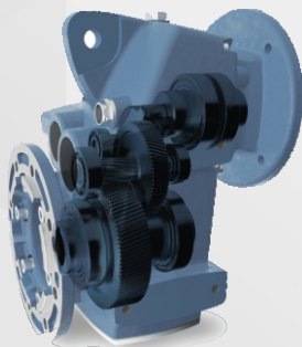
STON SERIES SHAFT MOUNTED
